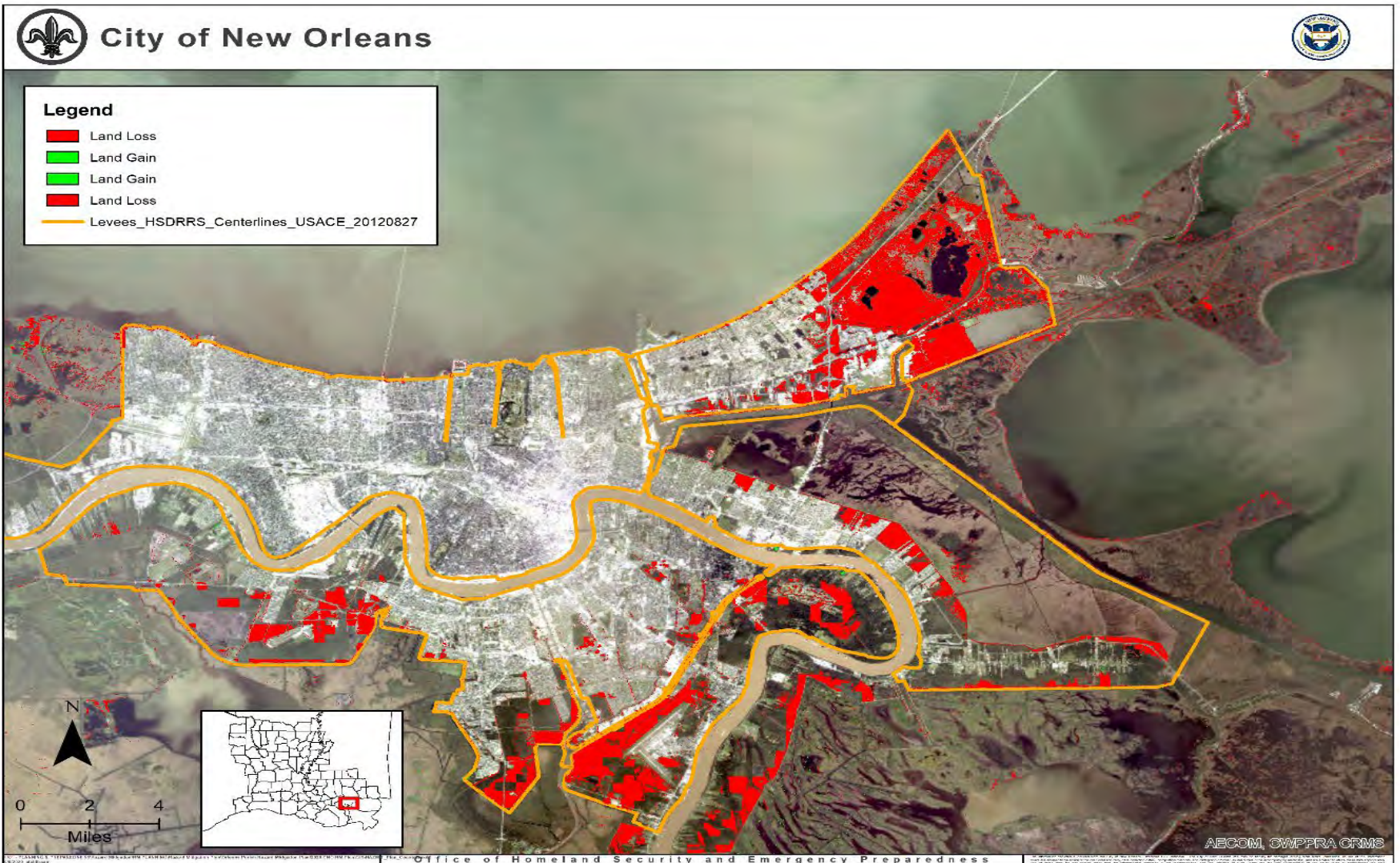
Figure 32: Low RSLR Scenario at Year 50
