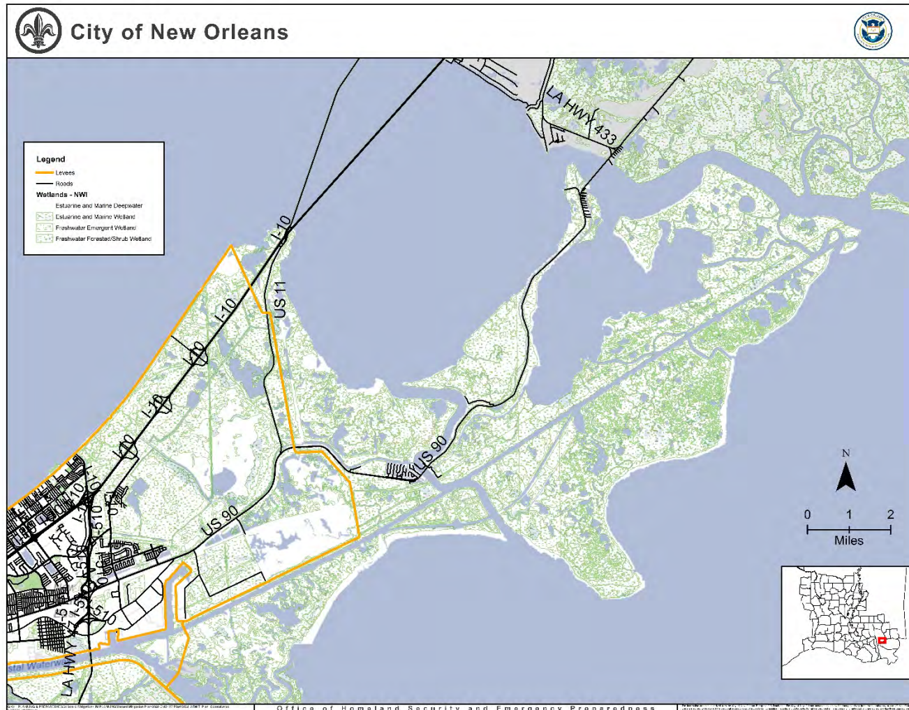
Figure 30: Location of Areas Subject to Coastal Erosion
