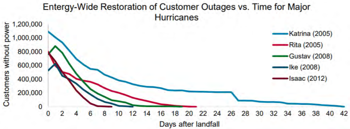
Figure 51: Customers Without Power Over Time for Past 5 Hurricanes Across All of Entergy’s Service Territory
