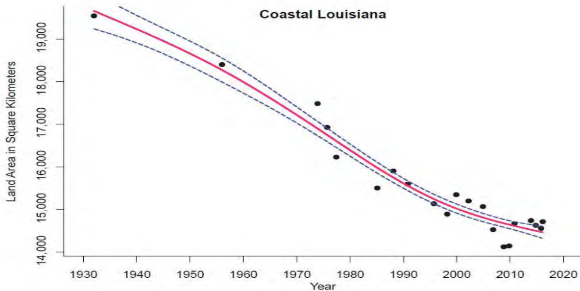
Figure 31: Change in Louisiana’s Coastal Wetland Areas, 1932 – 2016
