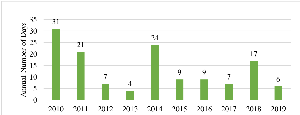
Figure 41: Number of Days of Temperature Less than 40°F
